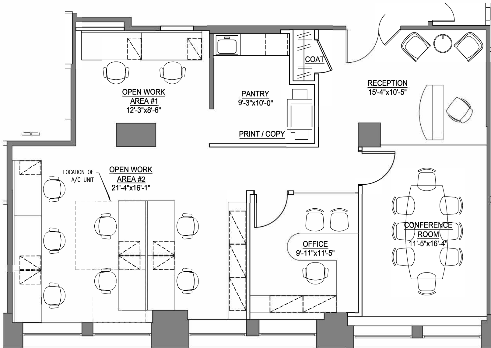
FLOOR PLAN - SUITE 505
