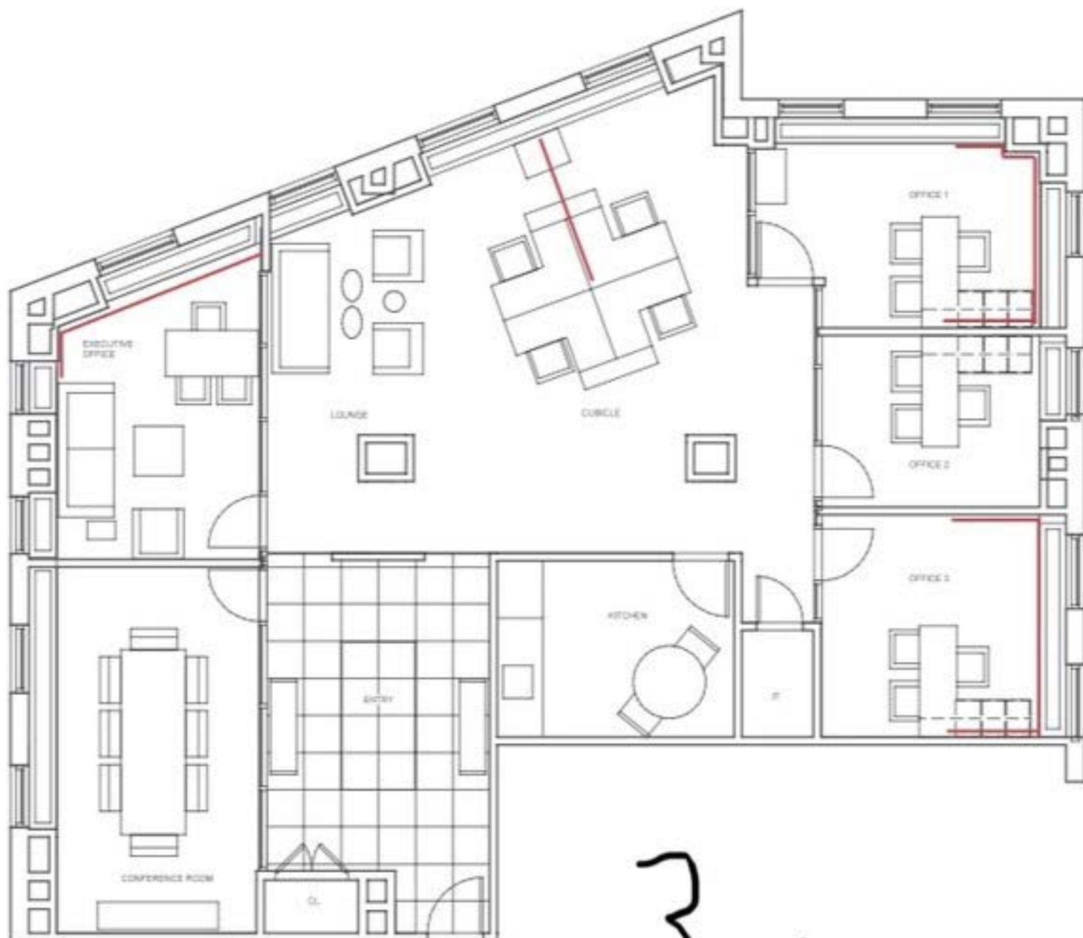
① FURNITURE PLAN 3/16" = 1'-0"
