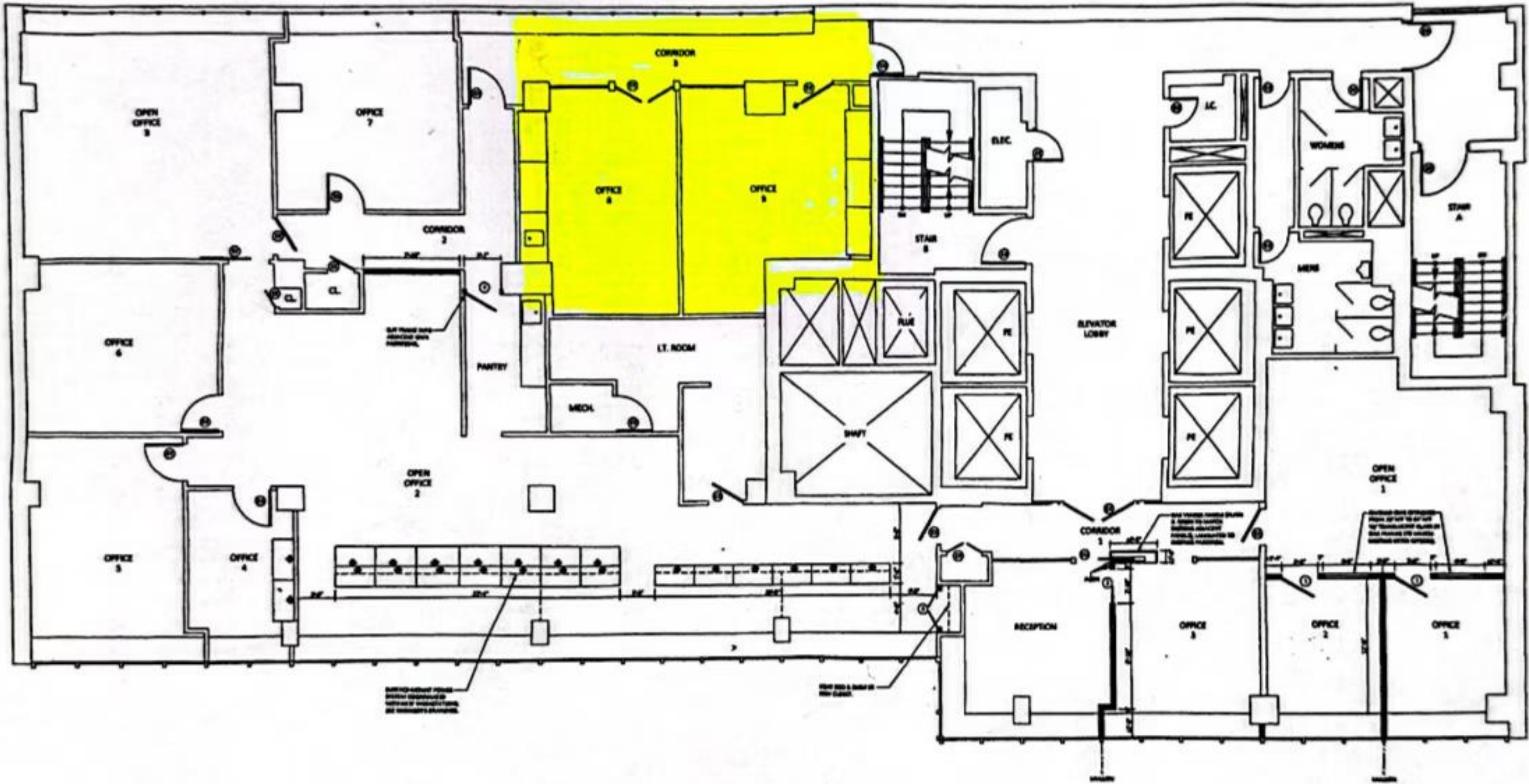
1 CONSTRUCTION PLAN : 14TH FLOOR 1/4" = 1'-0" NOTES: 1. NEW WALLS/DOORS SHALL BE IN ACCORDANCE WITH THE PROVISIONS OF THE IBC. 2. ALL WORK SHALL BE IN ACCORDANCE WITH THE IBC AND ALL APPLICABLE CODES. 3. ALL WORK SHALL BE IN ACCORDANCE WITH THE IBC AND ALL APPLICABLE CODES.
