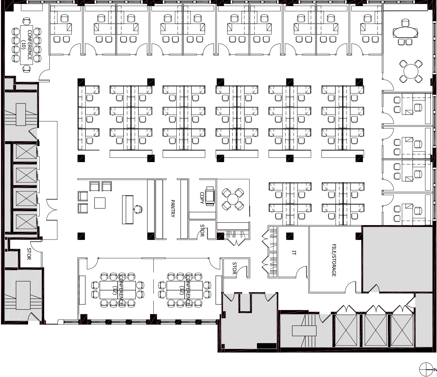
Office Intensive Layout
