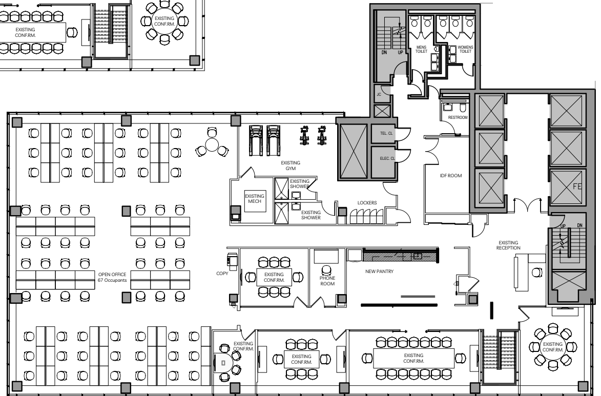
PROPOSED MODIFICATION PLAN
