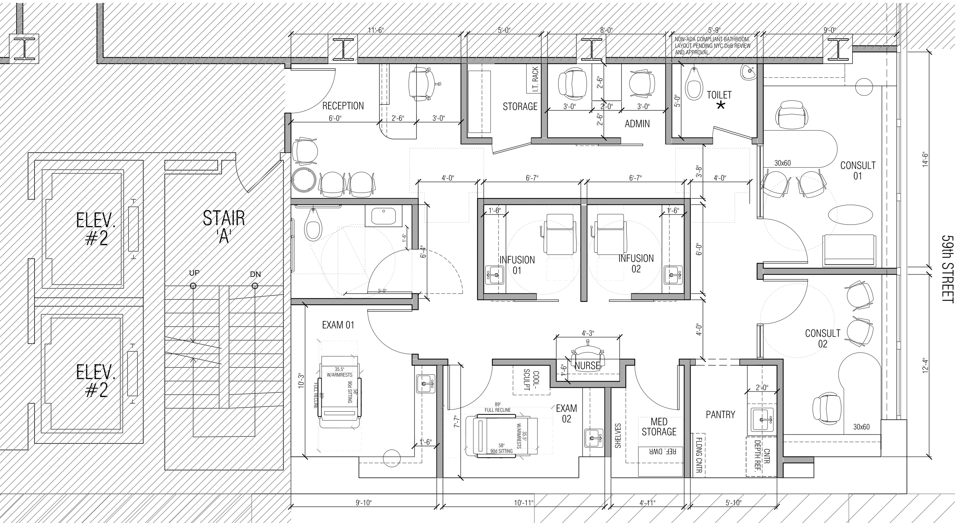
9th FLOOR PLAN - SUITE 900
