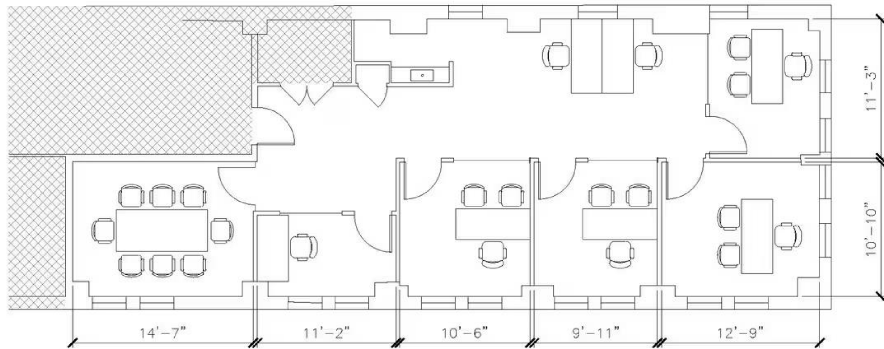
232 MADISON - 8TH FL - 800 PREBUILT SCALE: \frac{1}{8}" = 1'-0"
