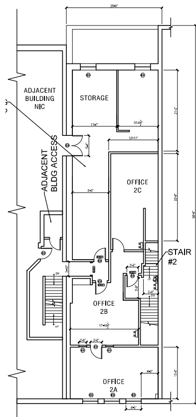
2ND FLOOR
