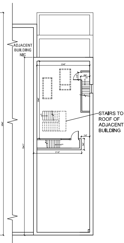
ROOF
