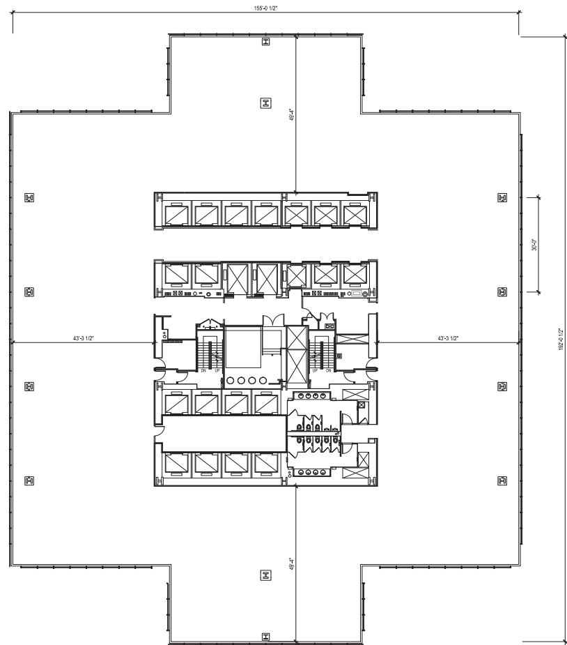
Typical Full Floor Core and Shell Plan
