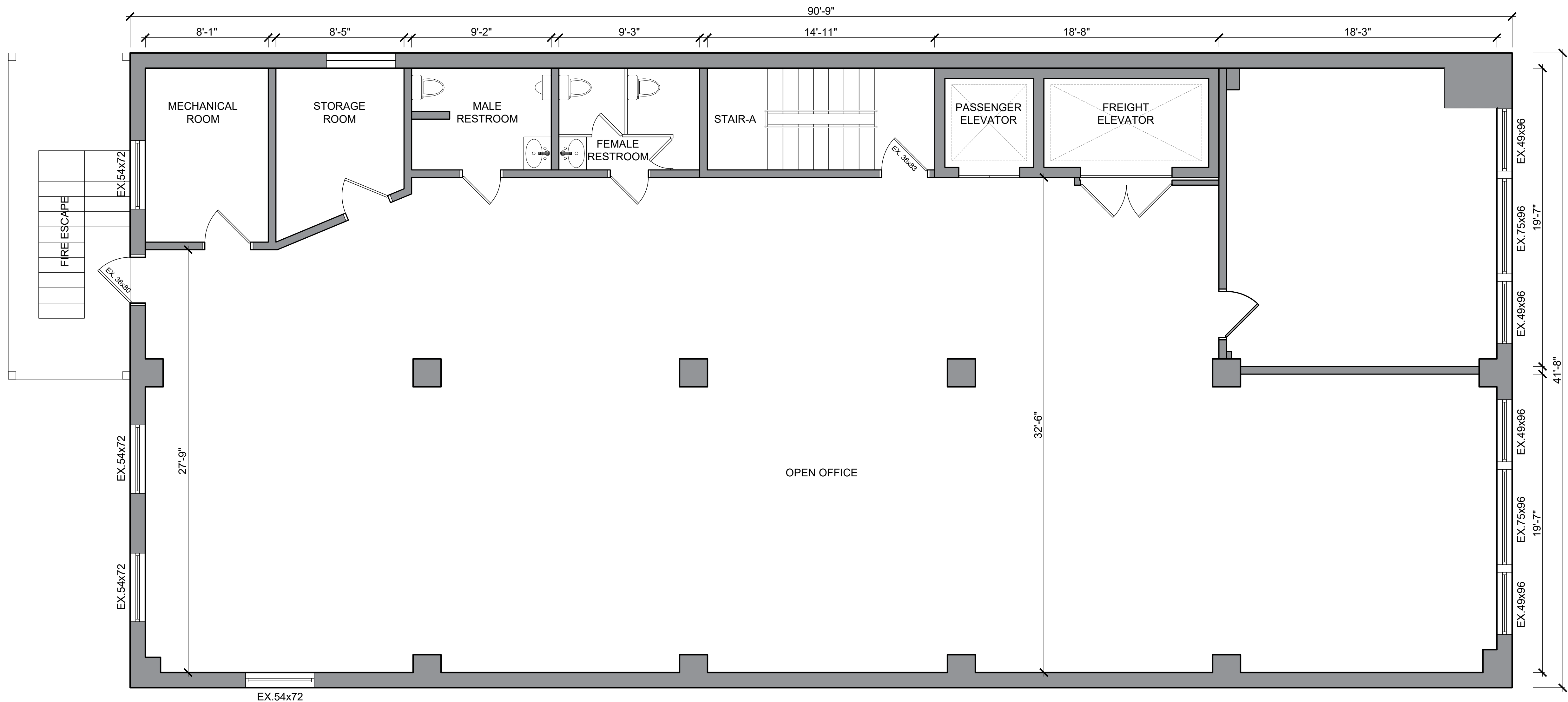
1 EXISTING 5th FLOOR PLAN SCALE: 1/4" = 1'-0"
