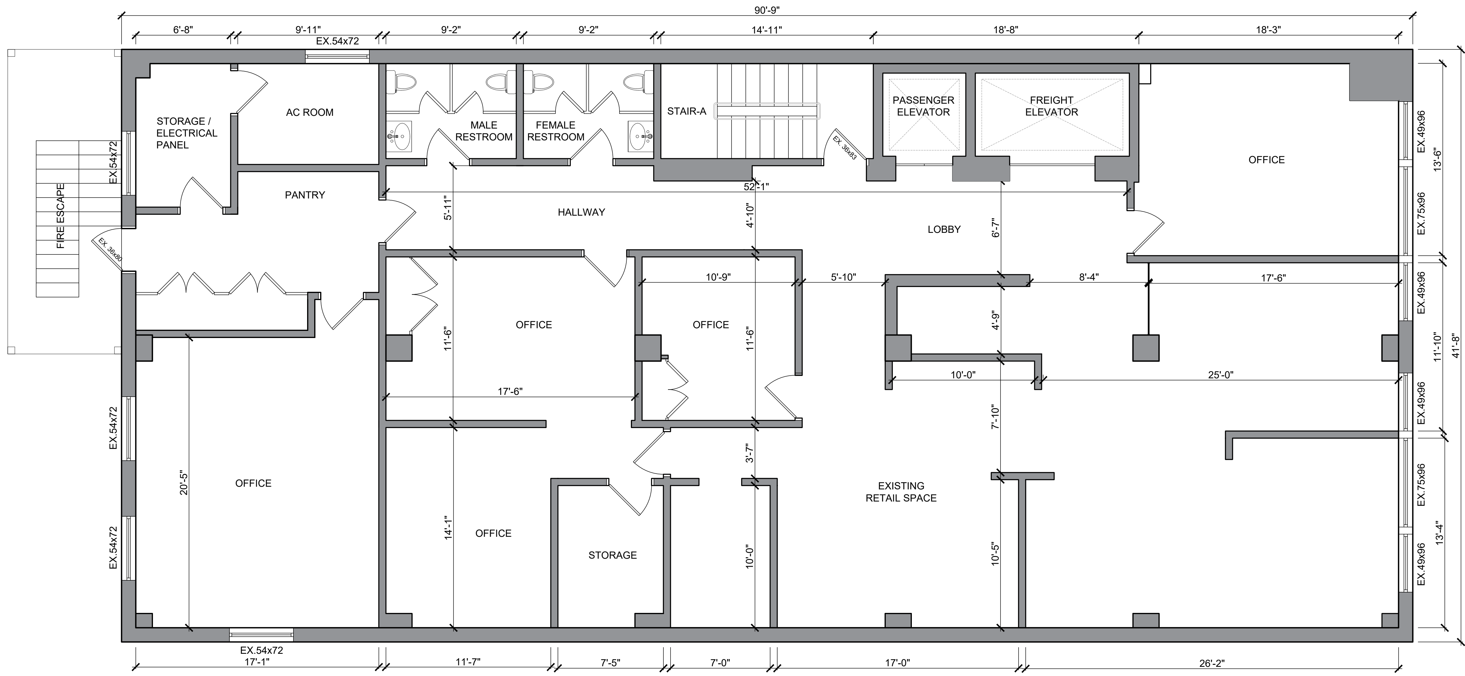
1 EXISTING 7th FLOOR PLAN SCALE: 1/4" = 1'-0"
