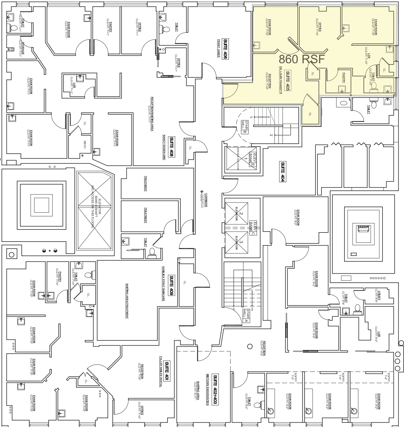
4TH FLOOR PLAN SCALE: 1/8"=1'-0"
