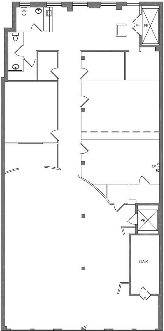
Entire 5th Floor As-Built
