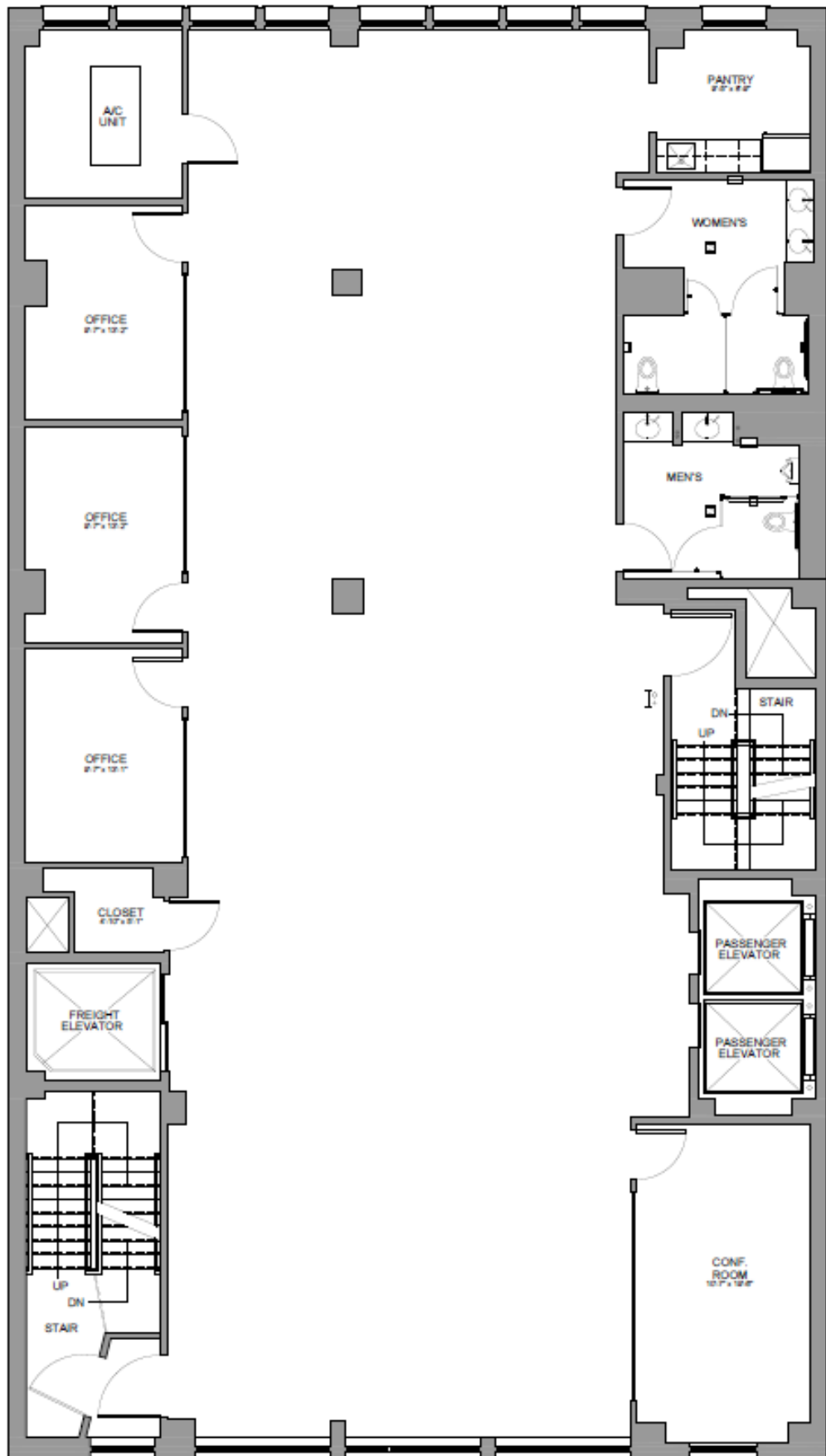
4th FLOOR - EXISTING CONDITIONS
