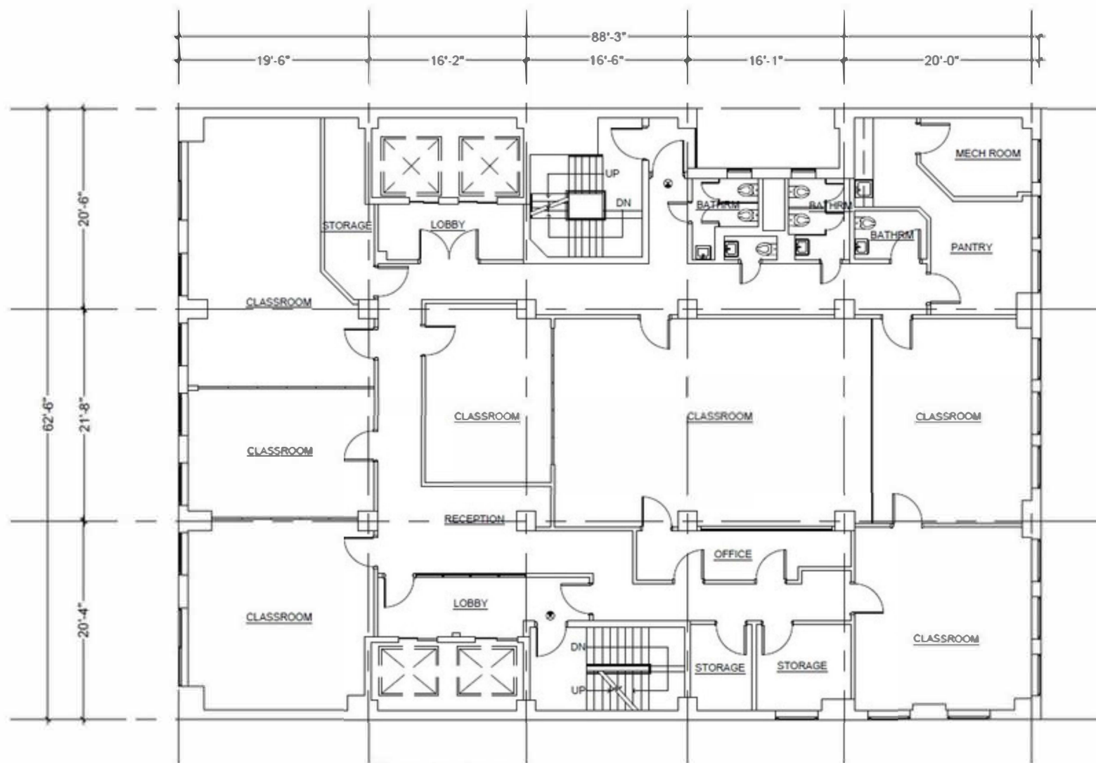
① 3RD FLOOR PLAN S/AE: 1/8"=1'-0"
